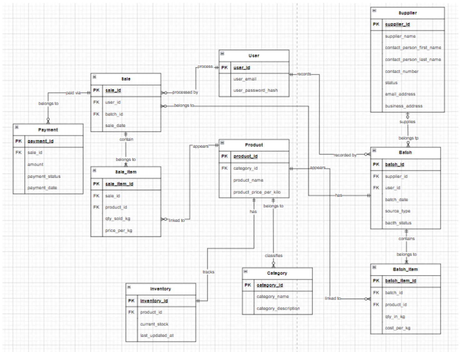
Figure 4: Full Blown ERD
