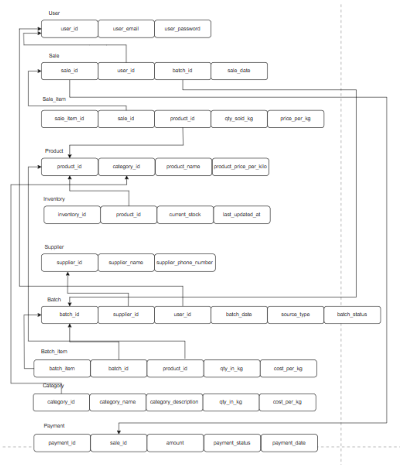
Figure 5: Entity Relation Mapping
